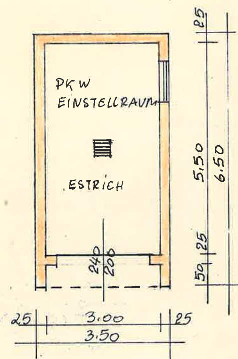
GARAGE GRUNDRISS
